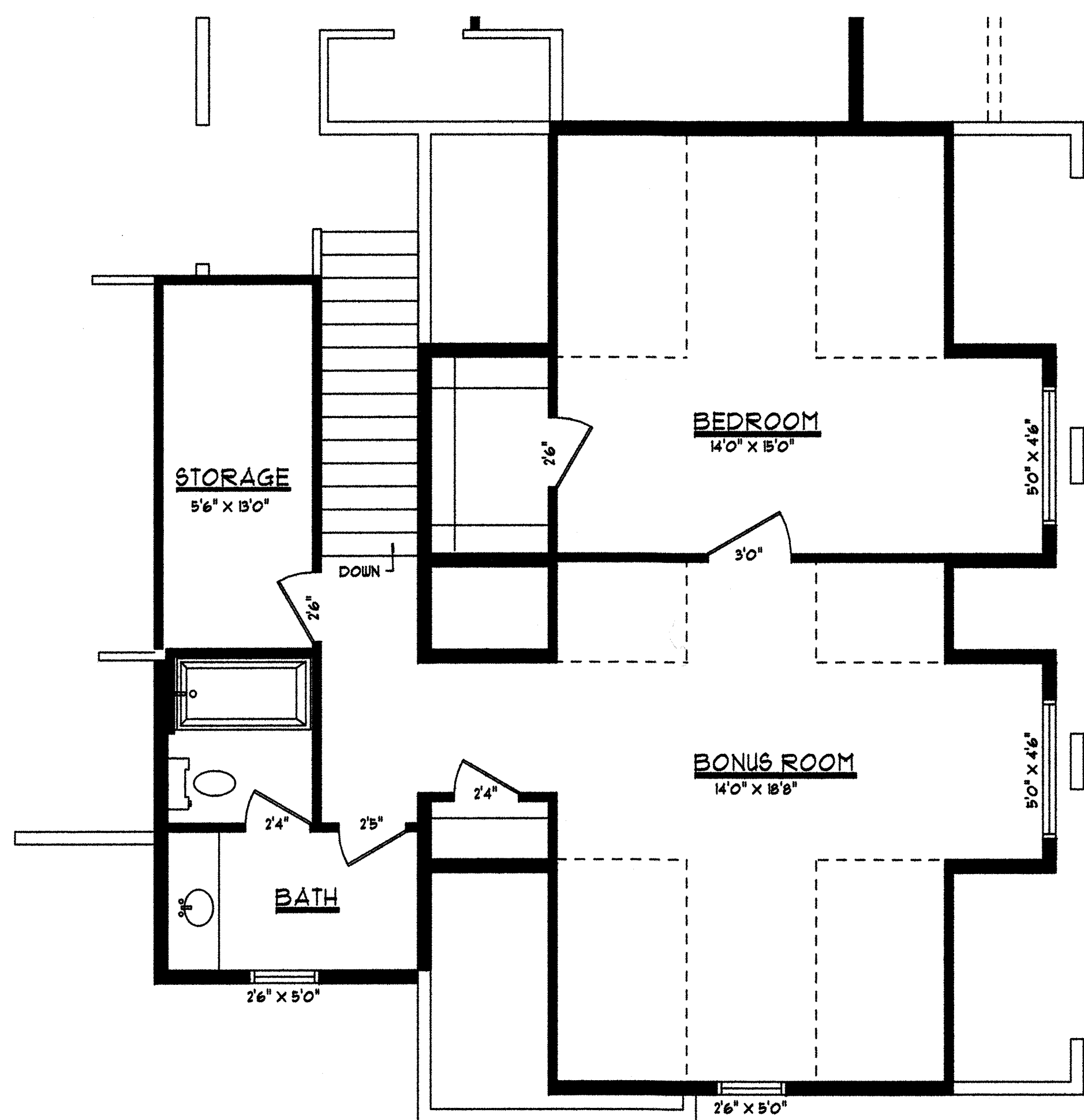
UPPER FLOOR PLAN
